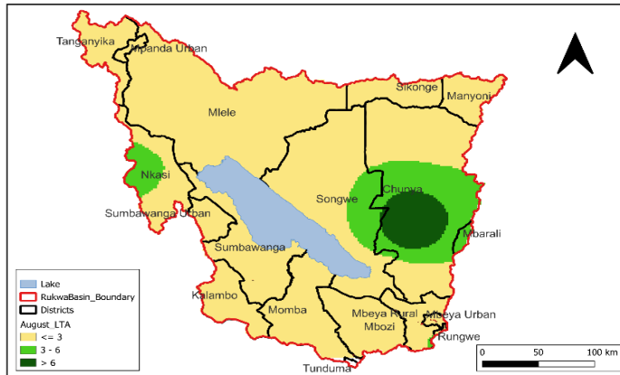
Figure 3: Long-term average rainfall distribution for August
