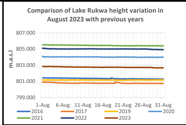
Figure 5: Water level in Lake Rukwa at Mbangala
